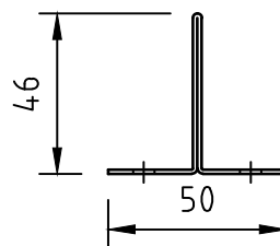
Profile 504 S steel 1,25 mm
