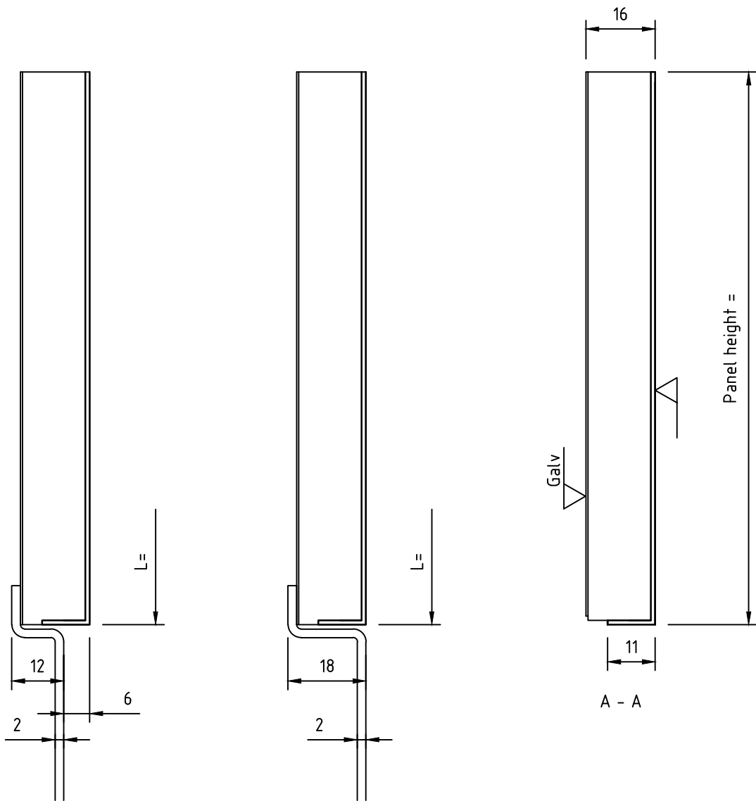
coaming alt. 1
