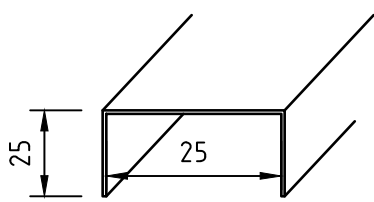
Top profile type 251 Galv 1,0 mm
