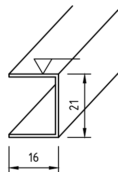
Connection profile type 421
