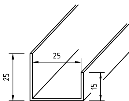
Bottom profile type 121 Galv 1,25 mm
