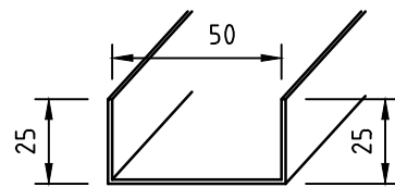
U profile Steel 1,25 mm
