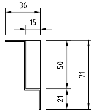
Steel profile Steel 1,25 mm
