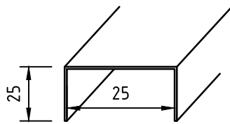
Top profile type 251 Galv 1,0 mm
