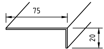
L profile type 466 Galv 1,25 mm
