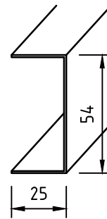
U profile type 461 Galv 1,25 mm
