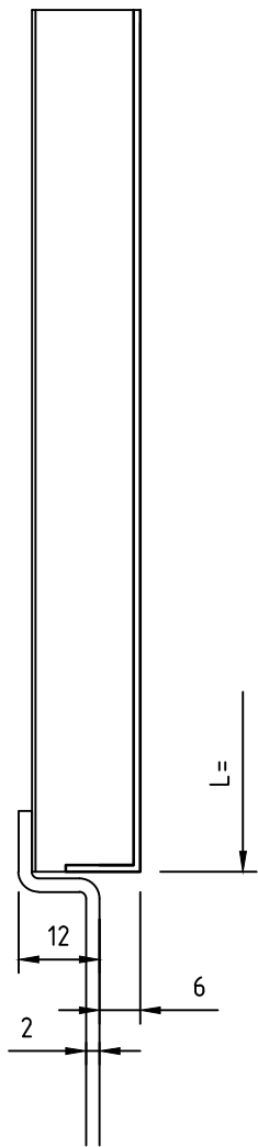
coaming alt. 1
