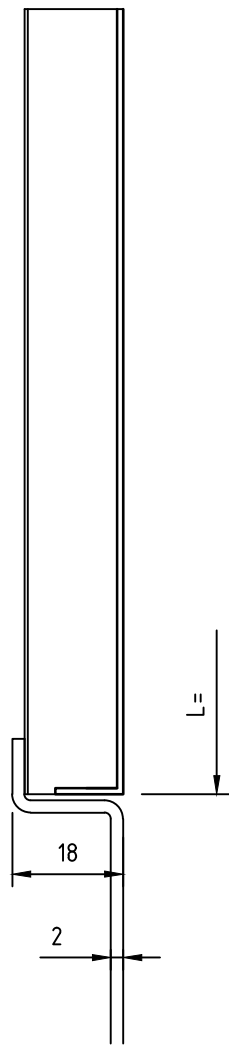
coaming alt. 2
