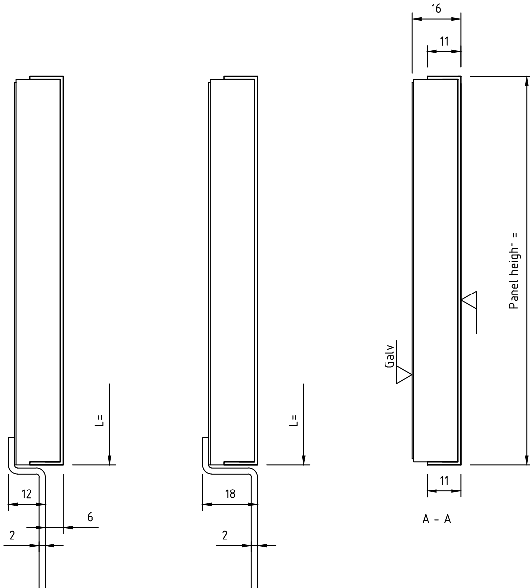
coaming alt. 1
